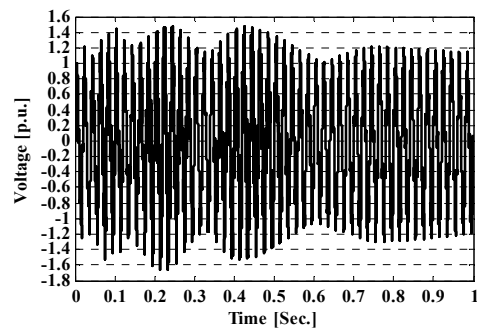
Figure 2. Voltage at bus 39 after switching of transformer.
