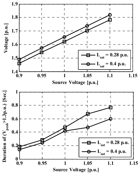
Figure 3. Overvoltage peak and duration at bus 39 as source voltage while line length 100 km, line capacitor 1.237e-8, switching angle 18° and remanent flux 0.8 p.u. L_{sat} is saturation curve slope.
