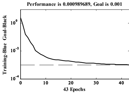
Figure 9. Squared error against epoch curve.
