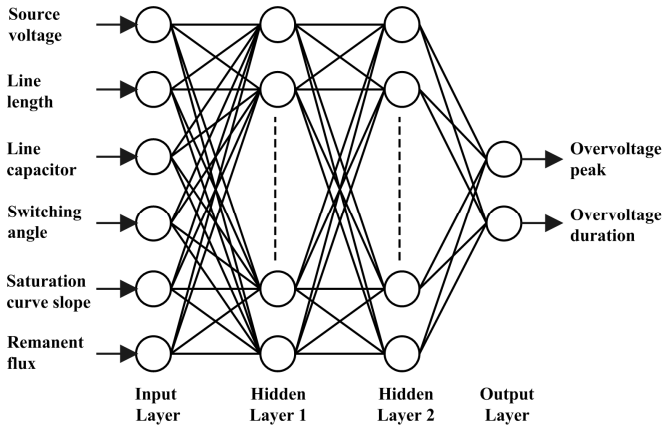
Figure 7. Proposed MLP-based ANN architecture.
