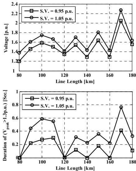
Figure 4. Overvoltage peak and duration at bus 39 as line length while line capacitor 1.237e-8, switching angle 18°, saturation curve slope 0.32 p.u. and remanent flux 0.8 p.u. S.V. is source voltage.
