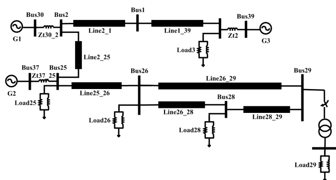
Figure 12. Studied system for case 2.
