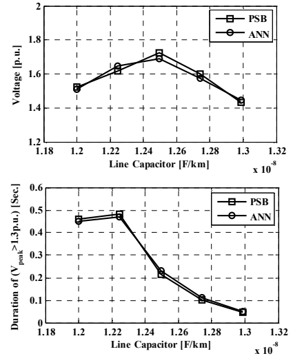
Figure 11. ANN output: overvoltage peak and duration at bus 39 simulated by ANN and PSB while source voltage 1 p.u., line length 100 km, switching angle 45°, saturation curve slope 0.32 p.u. and remanent flux 0.3 p.u.
