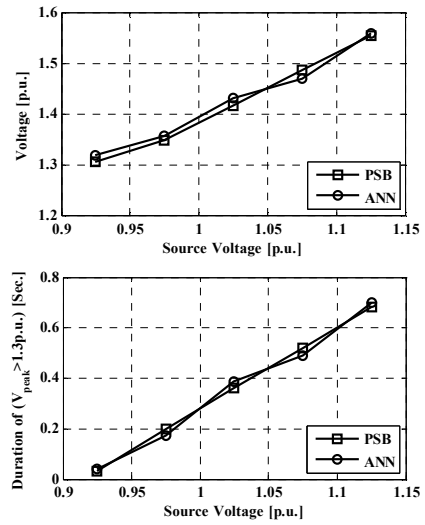
Figure 10. ANN output: overvoltage peak and duration at bus 39 simulated by ANN and PSB while line length 125 km, line capacitor 1.237e-8, switching angle 18°, saturation curve slope 0.38 p.u. and remanent flux 0.8 p.u.
