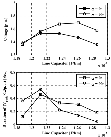
Figure 6. Overvoltage peak and duration at bus 39 as line capacitor while source voltage 1 p.u., line length 100 km, saturation curve slope 0.32 p.u. and remanent flux 0.8 p.u. \alpha is switching angle.
