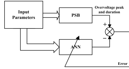
Figure 8. Supervised learning of ANN.
