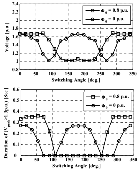
Figure 5. Overvoltage peak and duration at bus 39 as switching angle while source voltage 1 p.u., line length 100 km, line capacitor 1.237e-8 and saturation curve slope 0.32 p.u. \Phi_0 is remanent flux.
